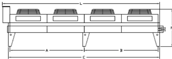
FRONT VIEW FEVK14 & FEVK24
