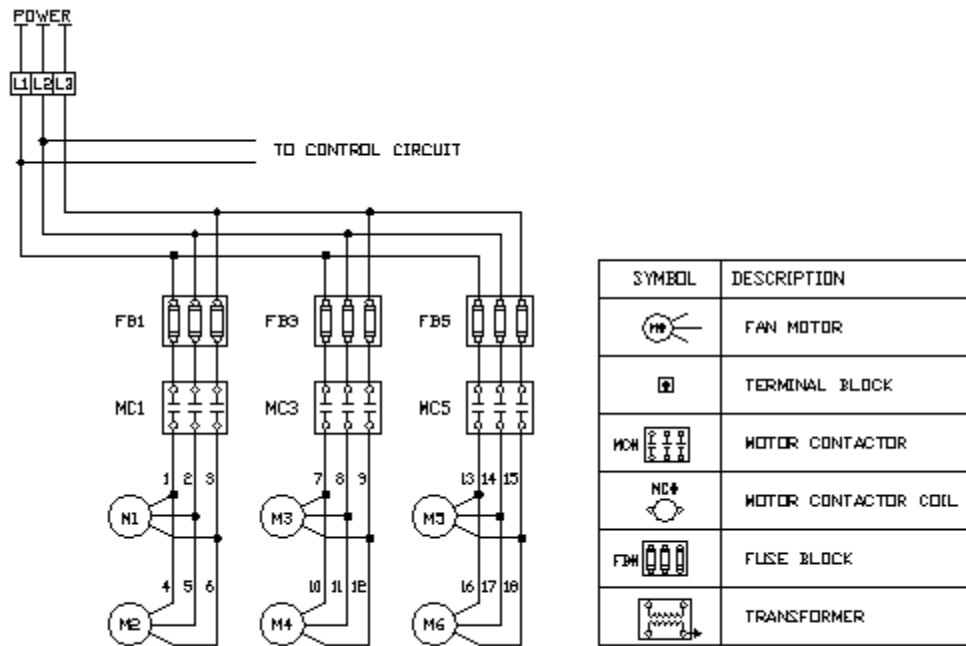
Figure 17 FAN MOTOR WIRING DIAGRAM (-331, -341)
