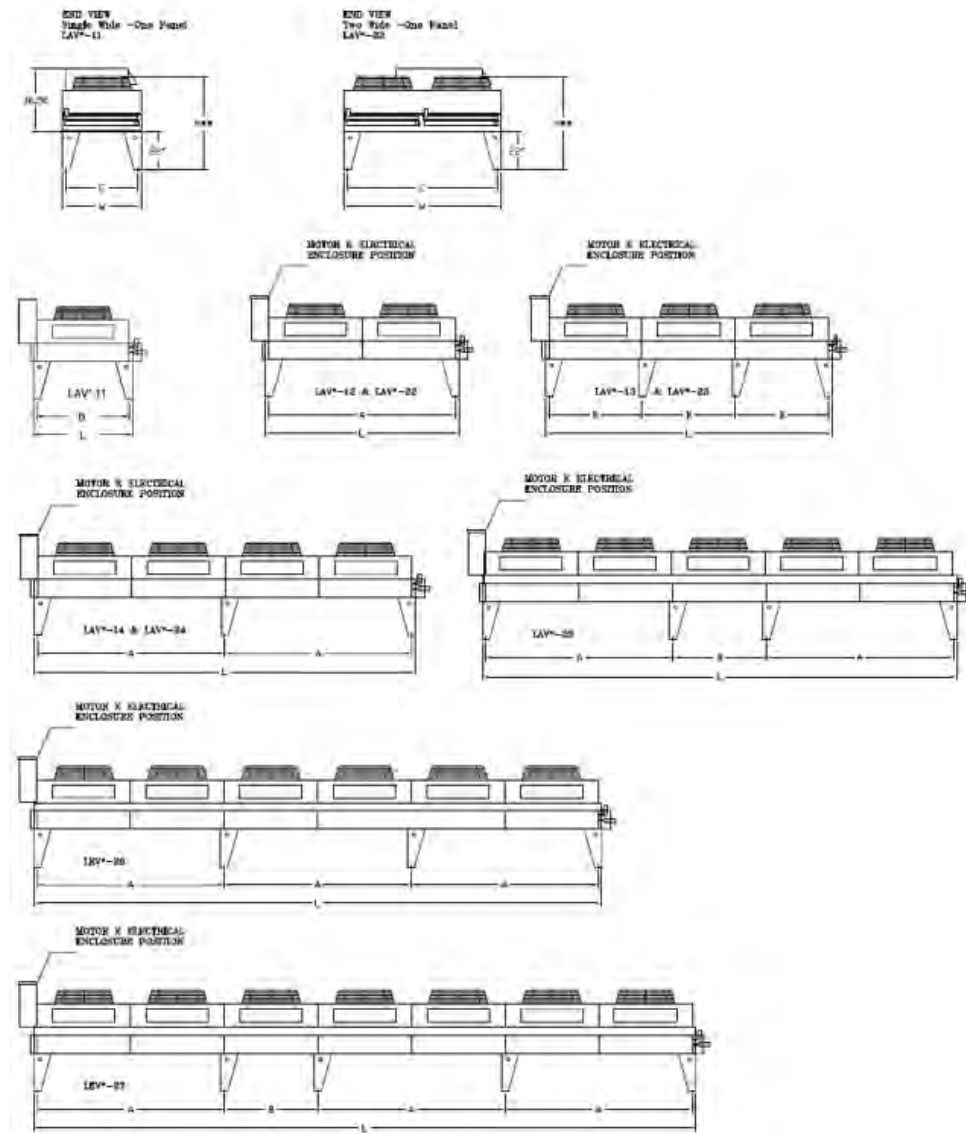
Figure 2 TWO WIDE UNIT DRAWINGS - K FAN MOTOR MODEL
