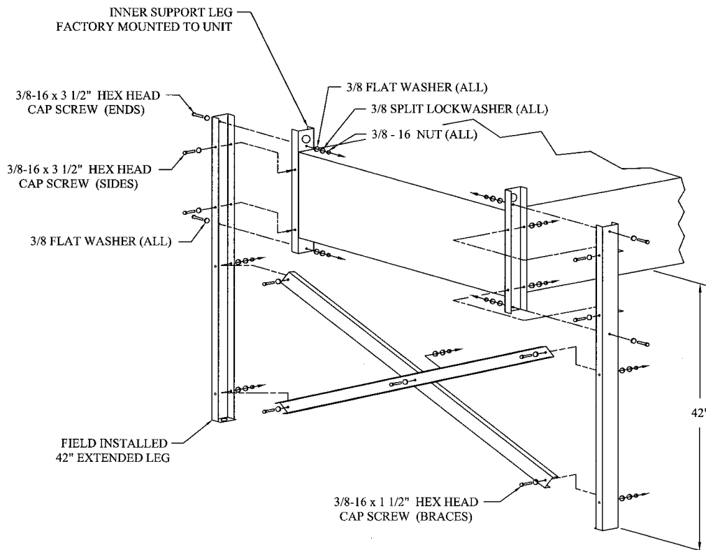
Figure 11 42" LEG & BRACING ASSEMBLY FOR 24" FAN UNITS
