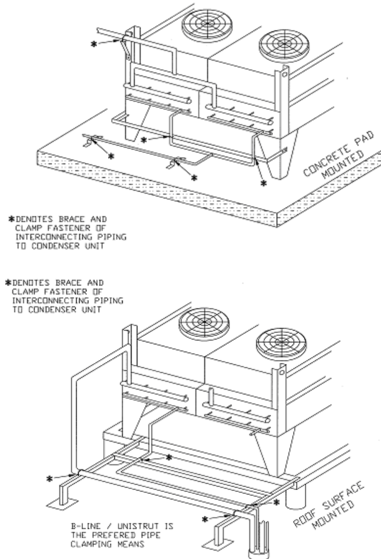
Figure 12 UNIT MOUNTING AND PIPING
