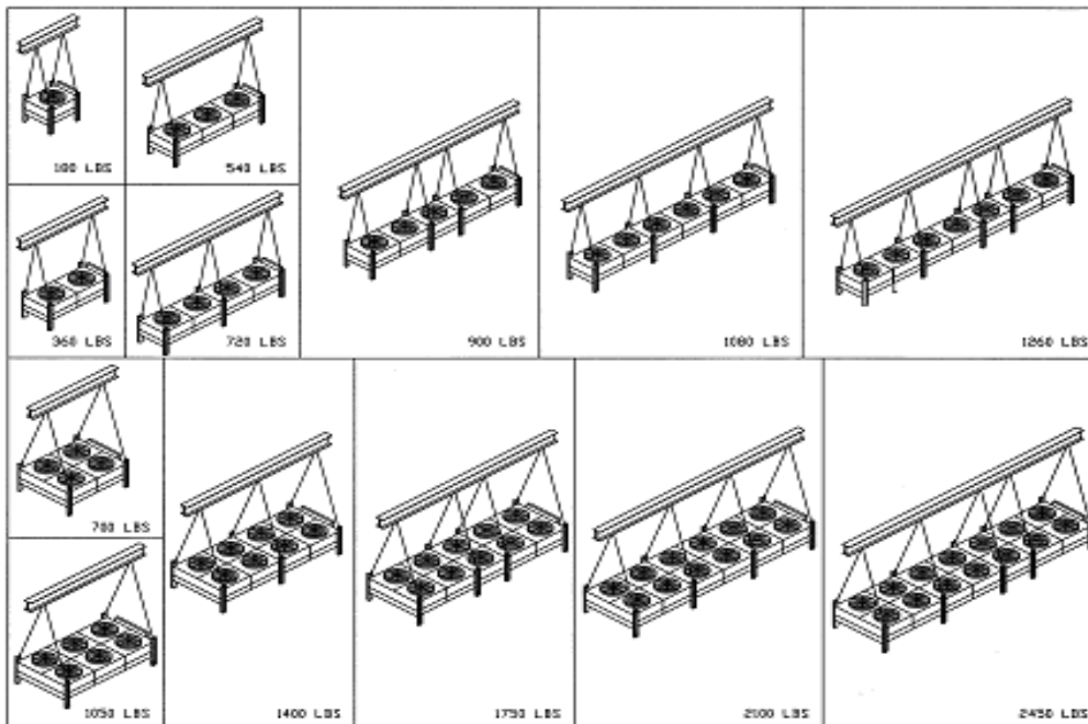
Figure 8 RIGGING FOR 24" FAN UNITS
