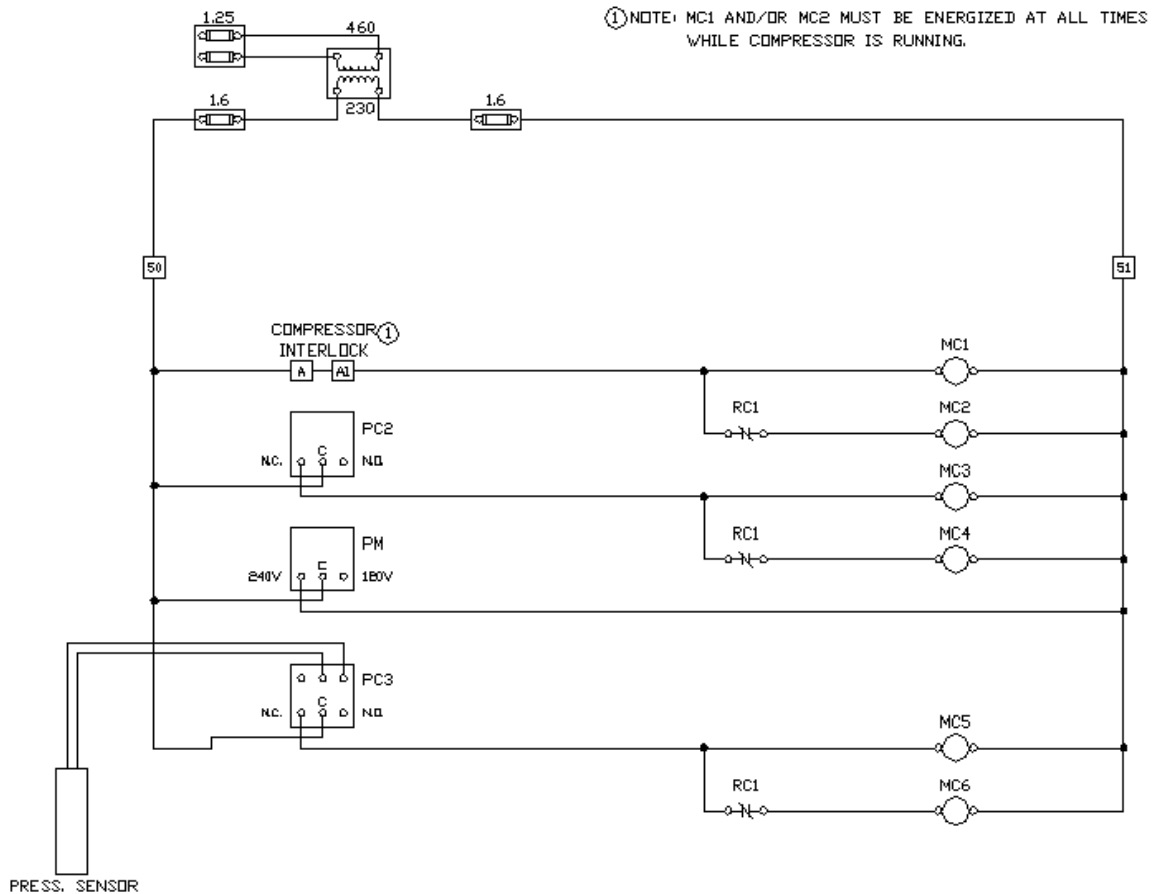
Figure 18 CONTROL CIRCUIT WIRING DIAGRAM (-355)
