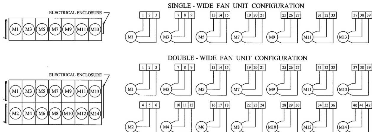
Figure 15 TERMINAL BLOCK ONLY WIRING DIAGRAMS (NC – C444)
