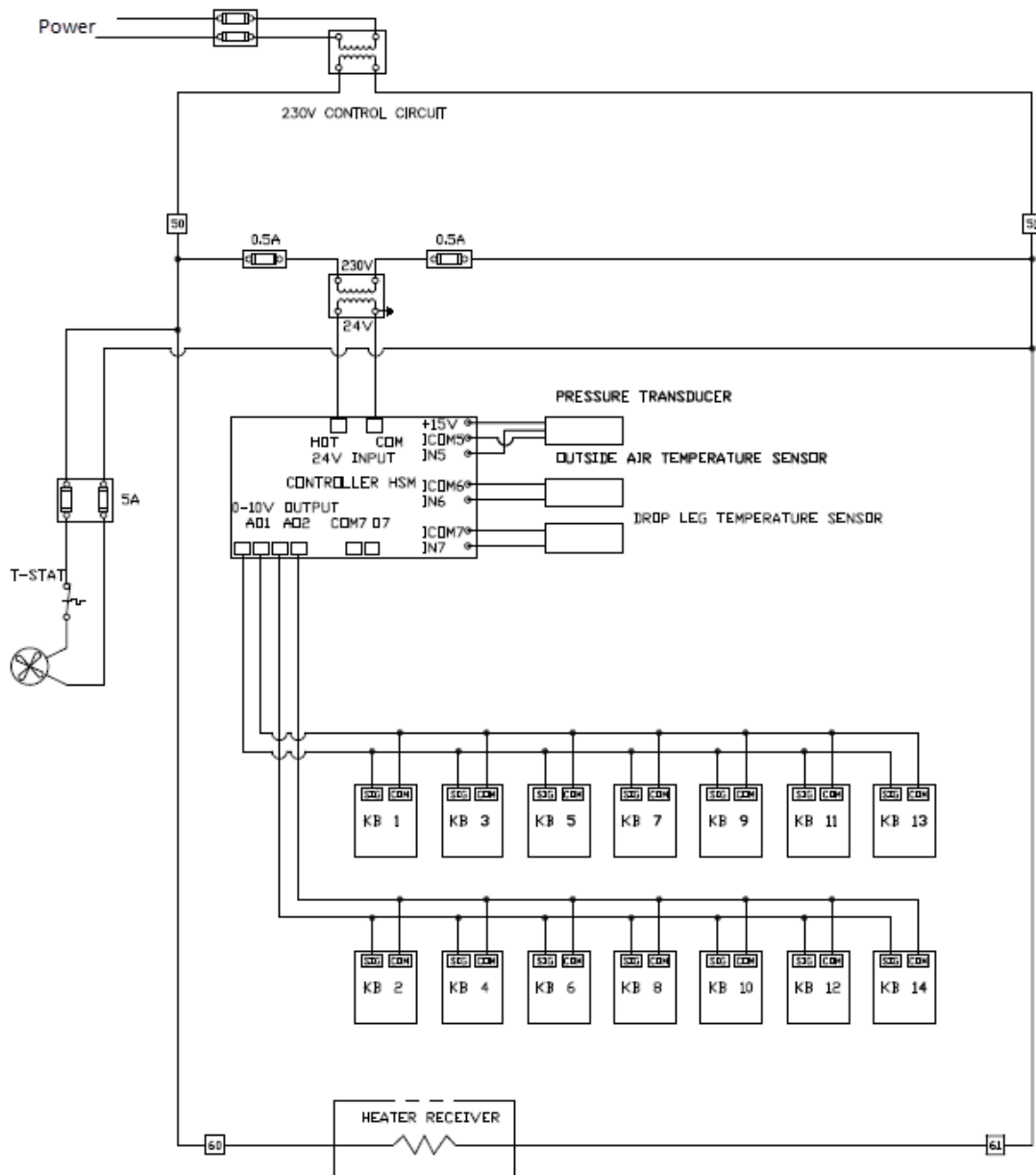
Figure 20 HUSSMANN CONTROLLER WIRING DIAGRAM
