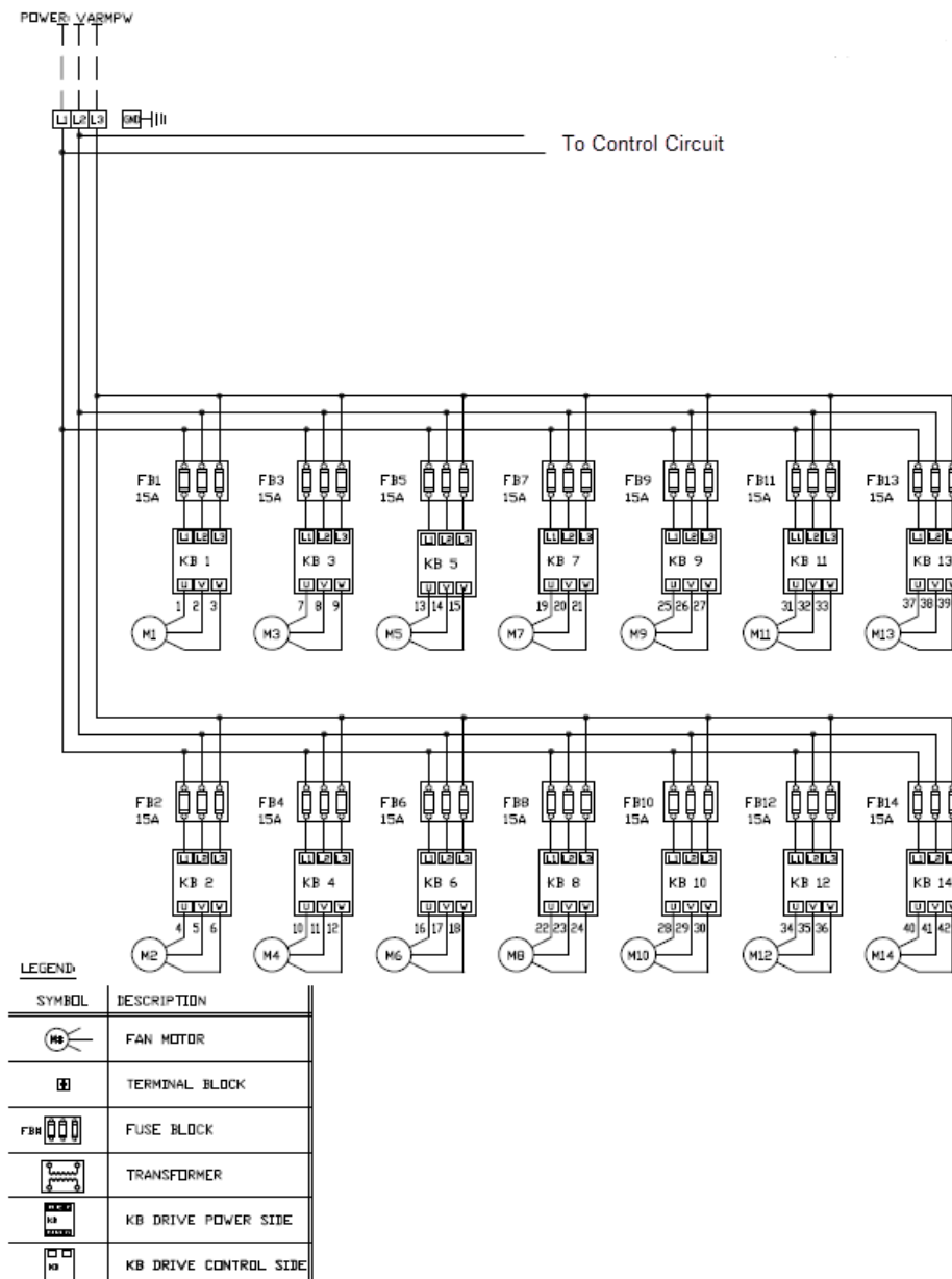
Figure 19 VARIABLE SPEED WIRING DIAGRAM
