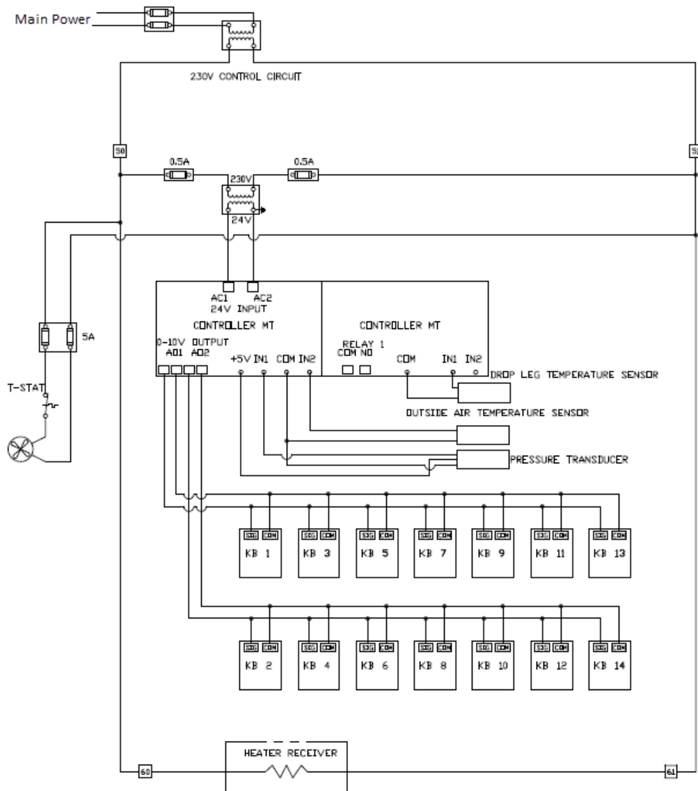
Figure 77 MICROTHERMO MT-722F MT-784A CONTROLLER WIRING DIAGRAM
