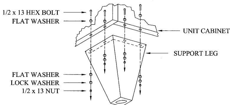
Figure 9 STANDARD 22" & 42" LEG ASSEMBLY
