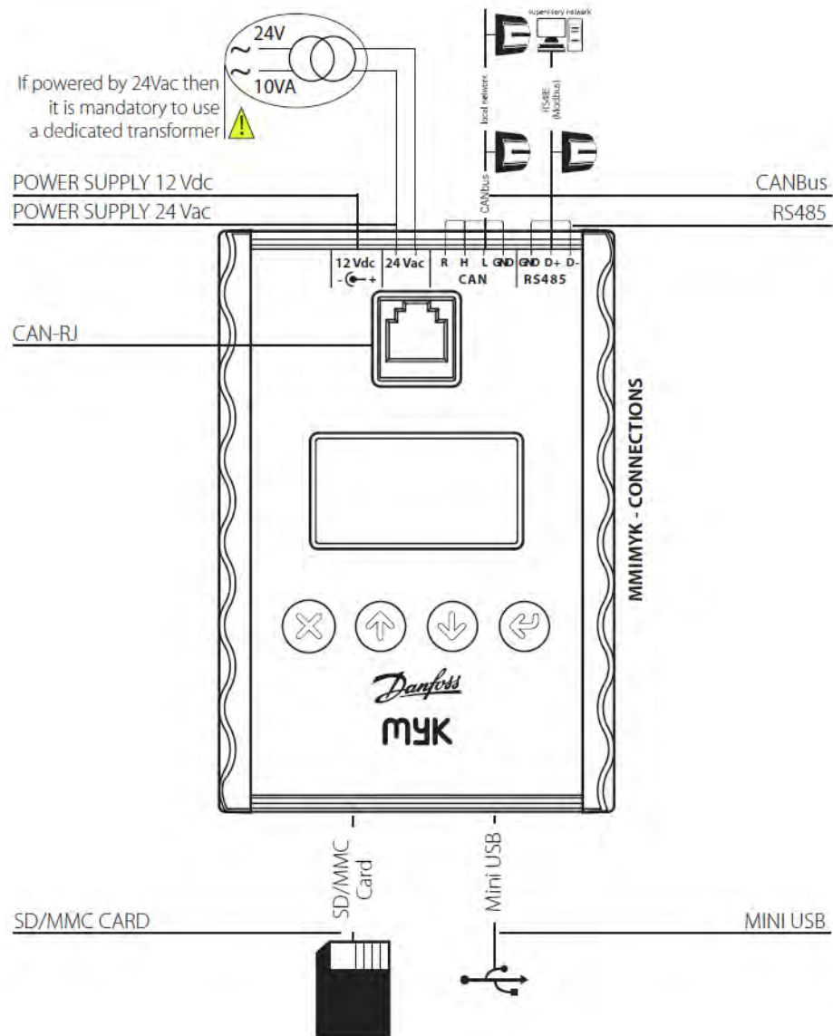
Figure 50 MMIMYK CONNECTION DIAGRAM
