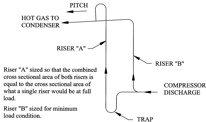
Figure 13 DOUBLE RISER DISCHARGE ARRANGEMENT
