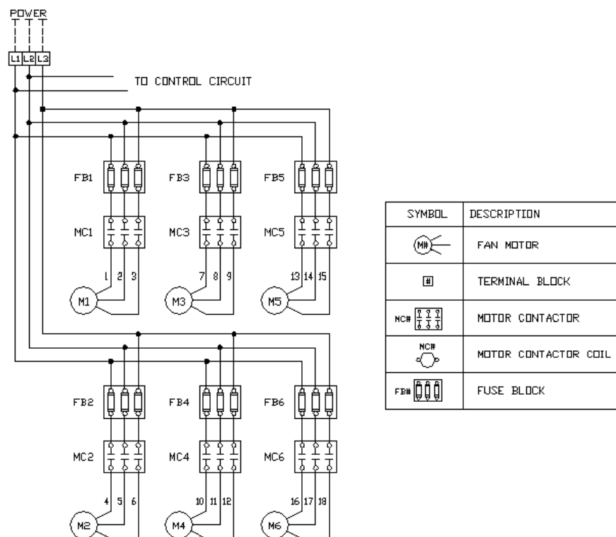
Figure 16 INDIVIDUAL FAN MOTOR WIRING DIAGRAM (-311, -411)
