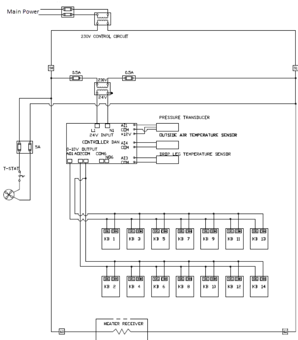
Figure 48 DANFOSS MCX06D CONTROLLER WIRING DIAGRAM
