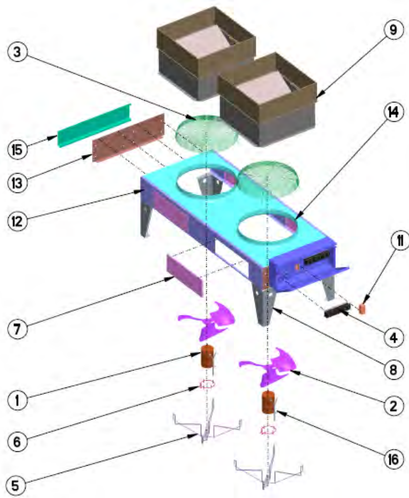
Figure 102 REPLACEMENT PARTS
